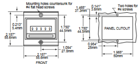
Panel Mount Depth: 2.377"/60.4mm
