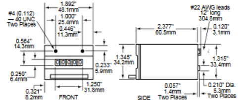
Back of Panel Mount Depth: 2.377"/60.5mm
