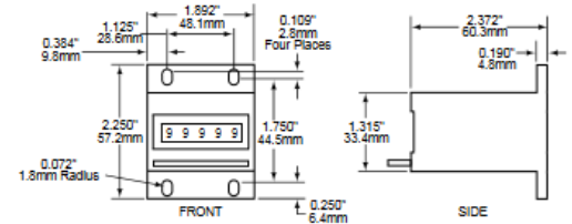
Base Mount Depth: 2.372"/60.3mm
